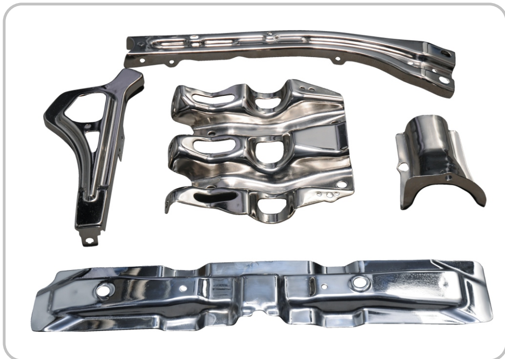
Metal Stampings for cowl bar assembly
